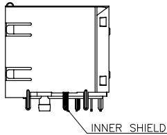
10118073-XXXAXXXLF (WITH INNER SHIELD)
