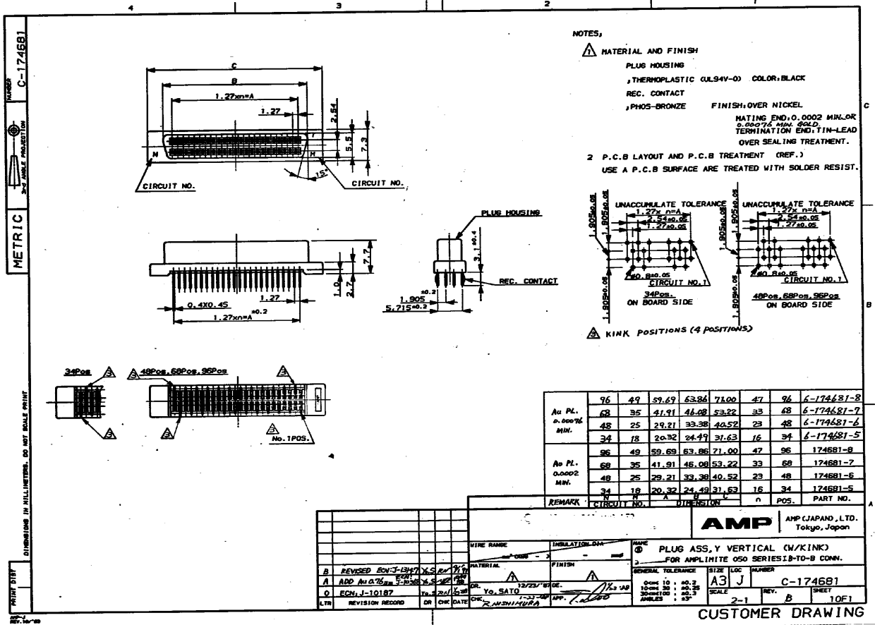
CUSTOMER DRAWING
