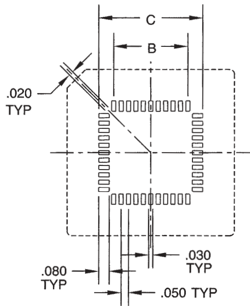
PCB LAYOUT
