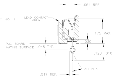
SECTION A-A ROTATED 90° CW SCALE 10:1 FOR -6, -7 & -8 ONLY
