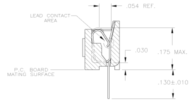
SECTION A-A ROTATED 90° CW SCALE 10:1 FOR -1, -2 & -3 ONLY
