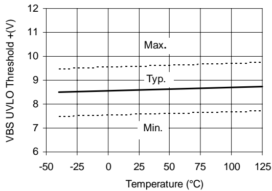
Figure 25 VBS Undervoltage Threshold (+) vs Temperature
