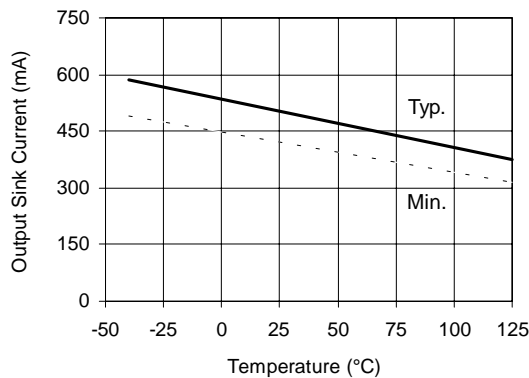
Figure 30A Output Sink Current vs Temperature
