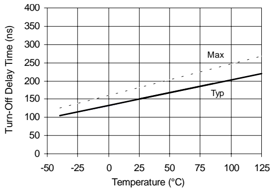
Figure 12A Turn-Off Time vs Temperature
