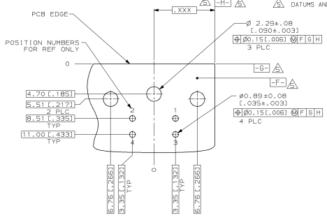
4 PIN PCB LAYOUT BOTTOM VIEW
