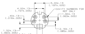
DETAIL D 4 PIN FACE
