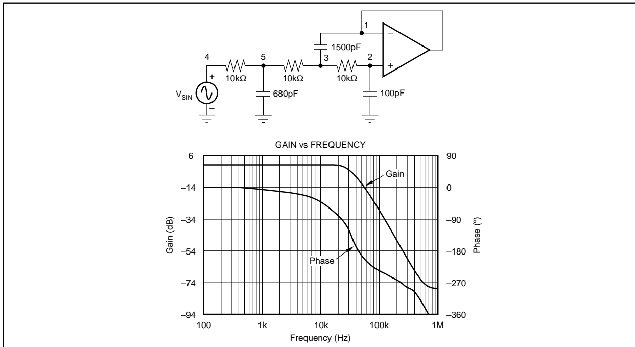
FIGURE 17. 3rd-Order LPF.
