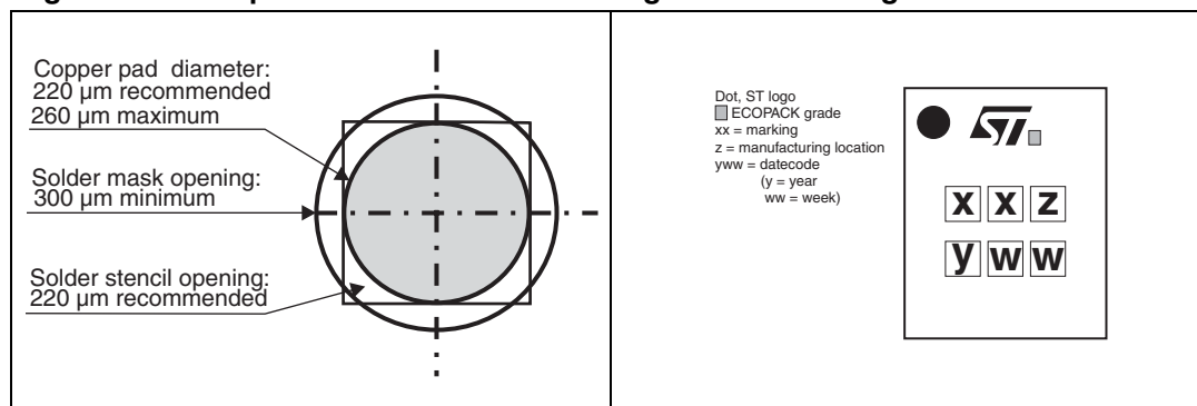
Figure 18. Footprint
