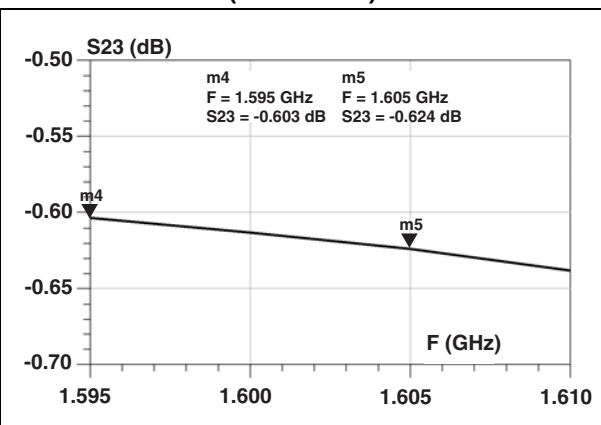
Figure 5. P2-P3 - S23 insertion loss in f2 band (GLONASS)
