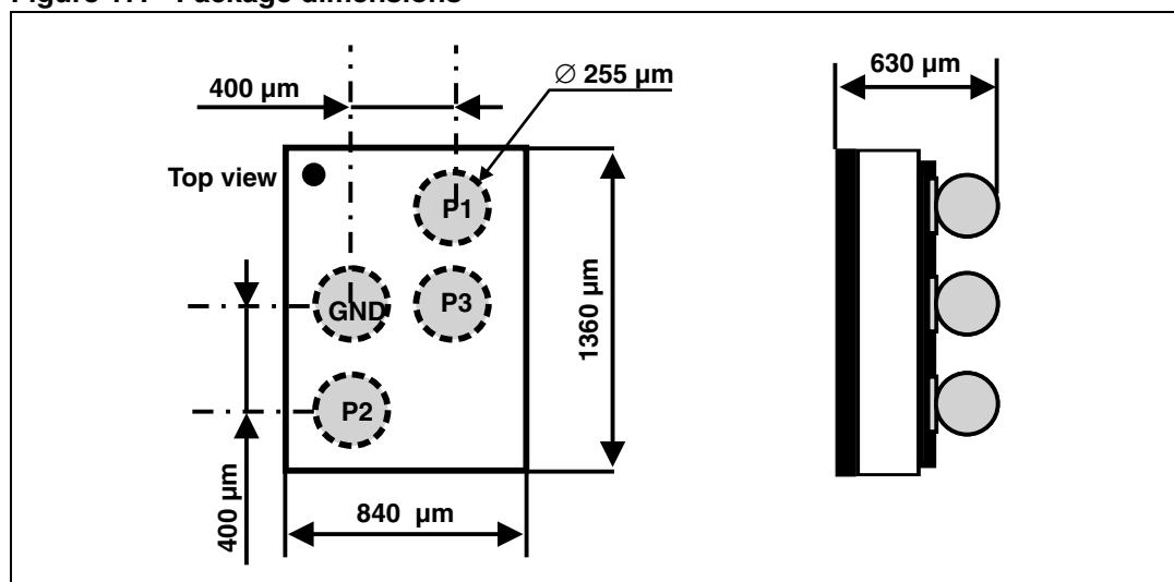
Figure 17. Package dimensions
