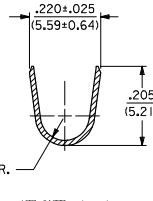
SECT. A-A
