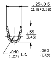
SECT. B-B
