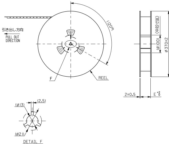
DETAIL F
