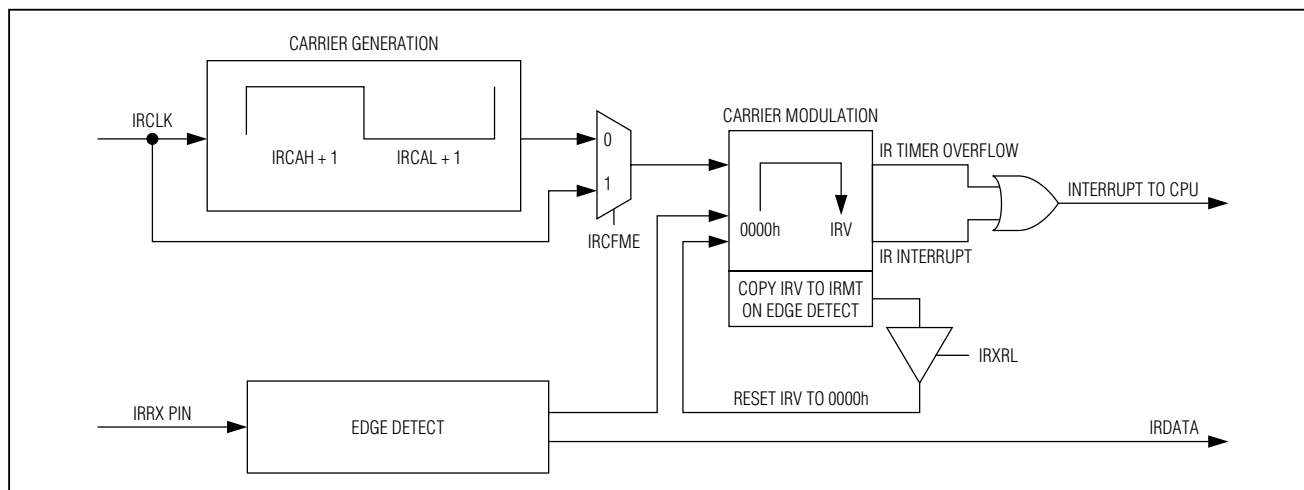
Figure 5. IR Capture
