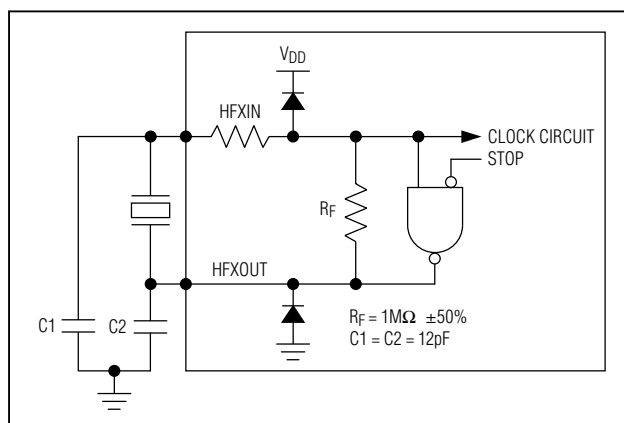
Figure 9. On-Chip Oscillator
