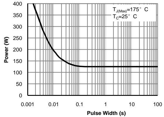
Figure 10: Single Pulse Power Rating Junction-to-Cs (Note F)
