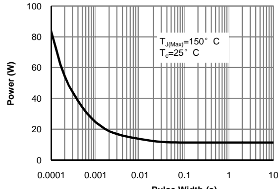
Figure 10: Single Pulse Power Rating Junction-to-Cz (Note F)
