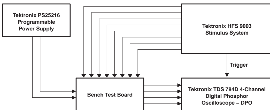
Figure 12. Equipment Setup
