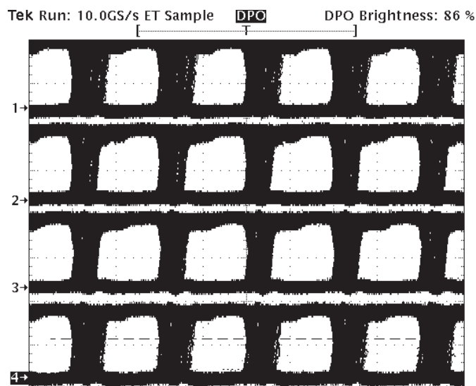
Figure 13. Typical Eye Pattern SN65LVDS32A 100 Mbit/s
