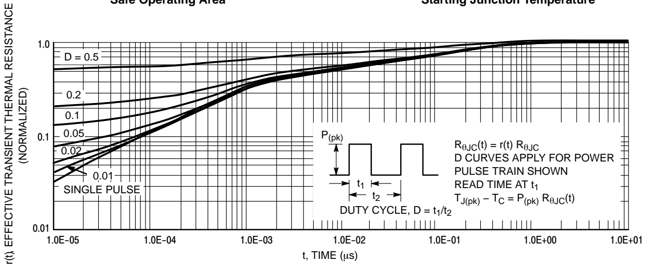
Figure 13. Thermal Response
