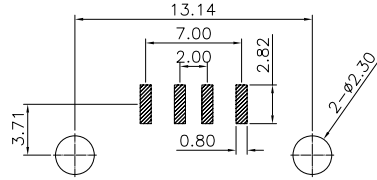
RECOMMENDED P. C. B. PATTERN LAYOUT
