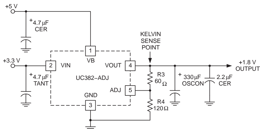
Figure 8. Typical UC382-ADJ Application
