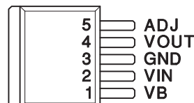
5-PIN TO-263 TD PACKAGE (TOP VIEW)
