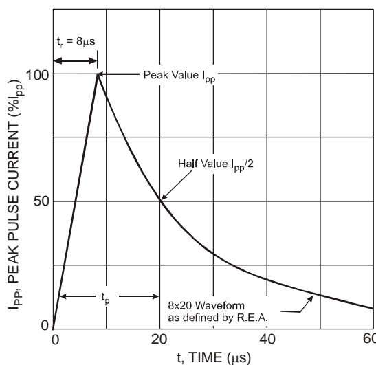
Fig. 2 Pulse Waveform
