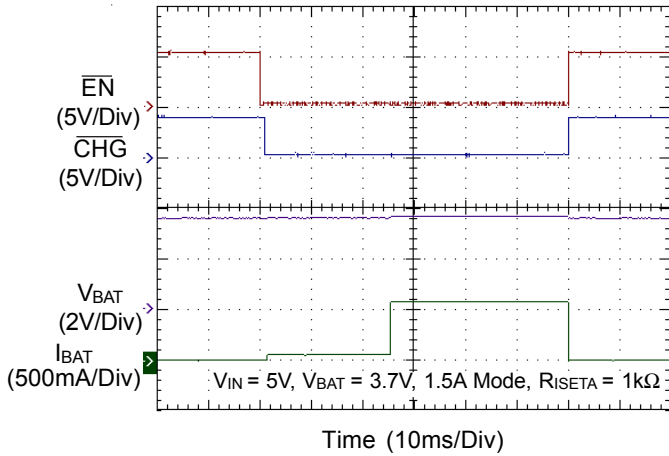
Charger Detect Sequence
