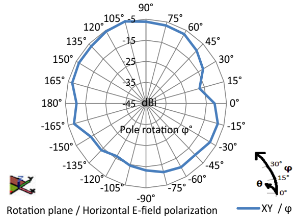
Fig. 4 - VJ5301M868MXBSR XY Radiation Pattern
