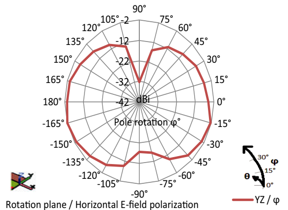
Fig. 5 - VJ5301M868MXBSR YZ Radiation Pattern
