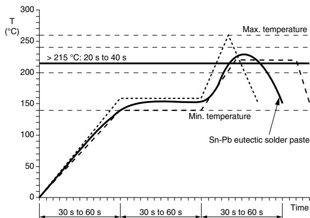
Fig. 8 - Soldering IR Reflow with SnPb Solder
