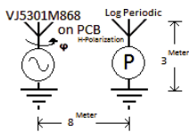
Fig. 3 - VJ5301M868 PCB Mounting and Coordinate Directions
