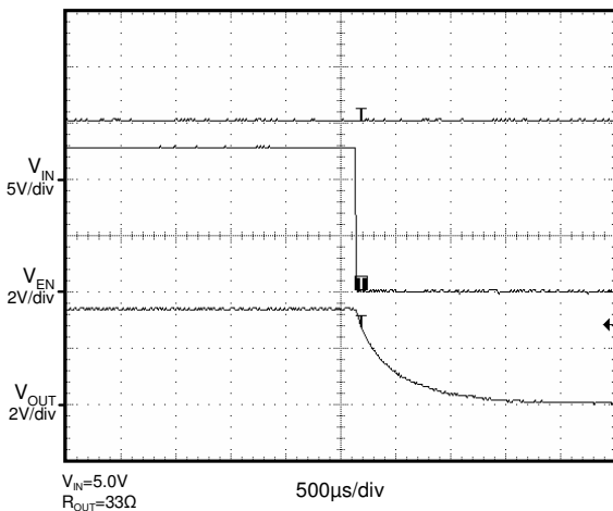
Shutdown (Disable) ( V_{OUT}=3.3V )
