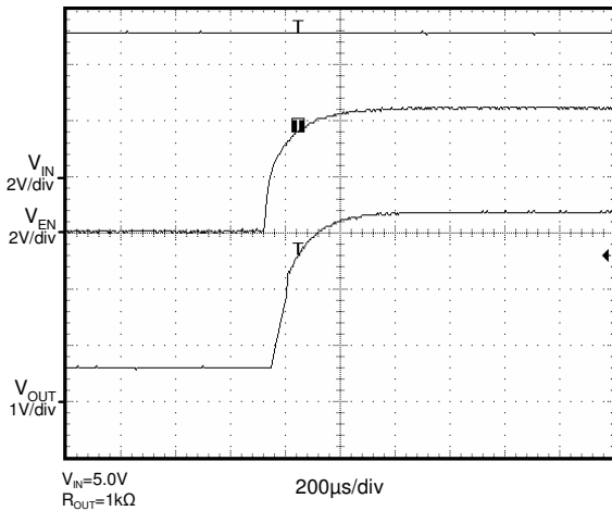
Start Up into Pre-Bias Output (Enable)
