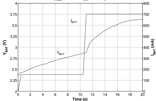
Re-Charge Cycle Battery Voltage and Current
