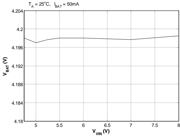
CV Line Regulation
