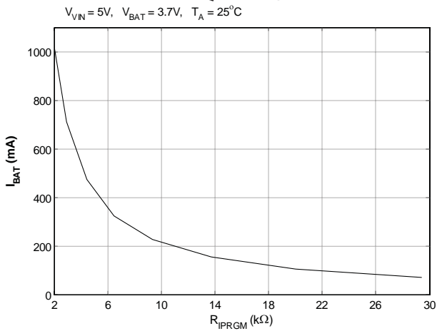
I_{\text{FQ}} vs. R_{\text{IPRGM}}
