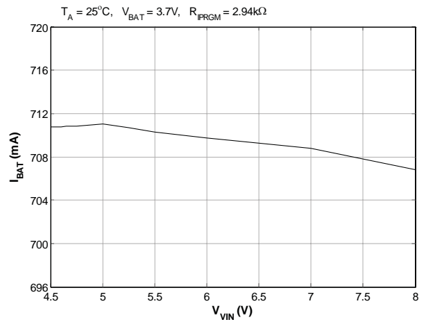
CC FQ Line Regulation
