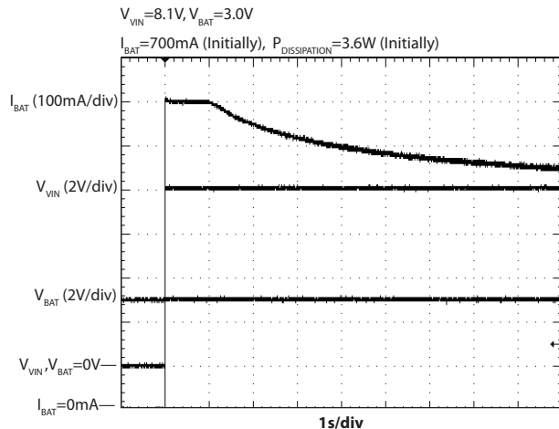
Figure 4 — Thermal Limiting Example
