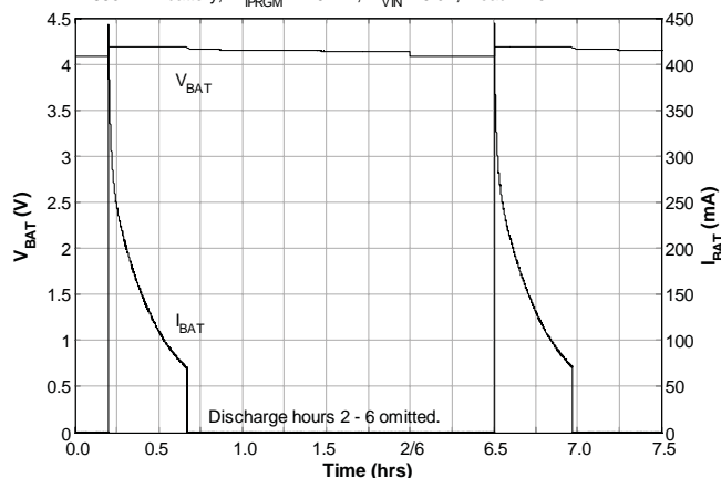
Re-Charge Cycle Battery Voltage and Current
