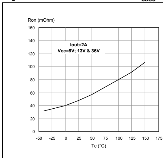
Figure 16. On-state resistance vs T case
