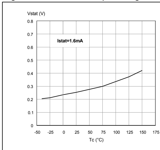
Figure 10. Status low output voltage
