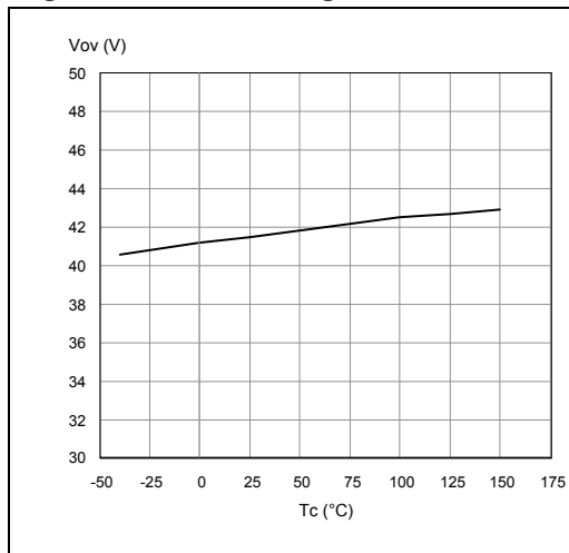
Figure 14. Turn-on voltage slope
