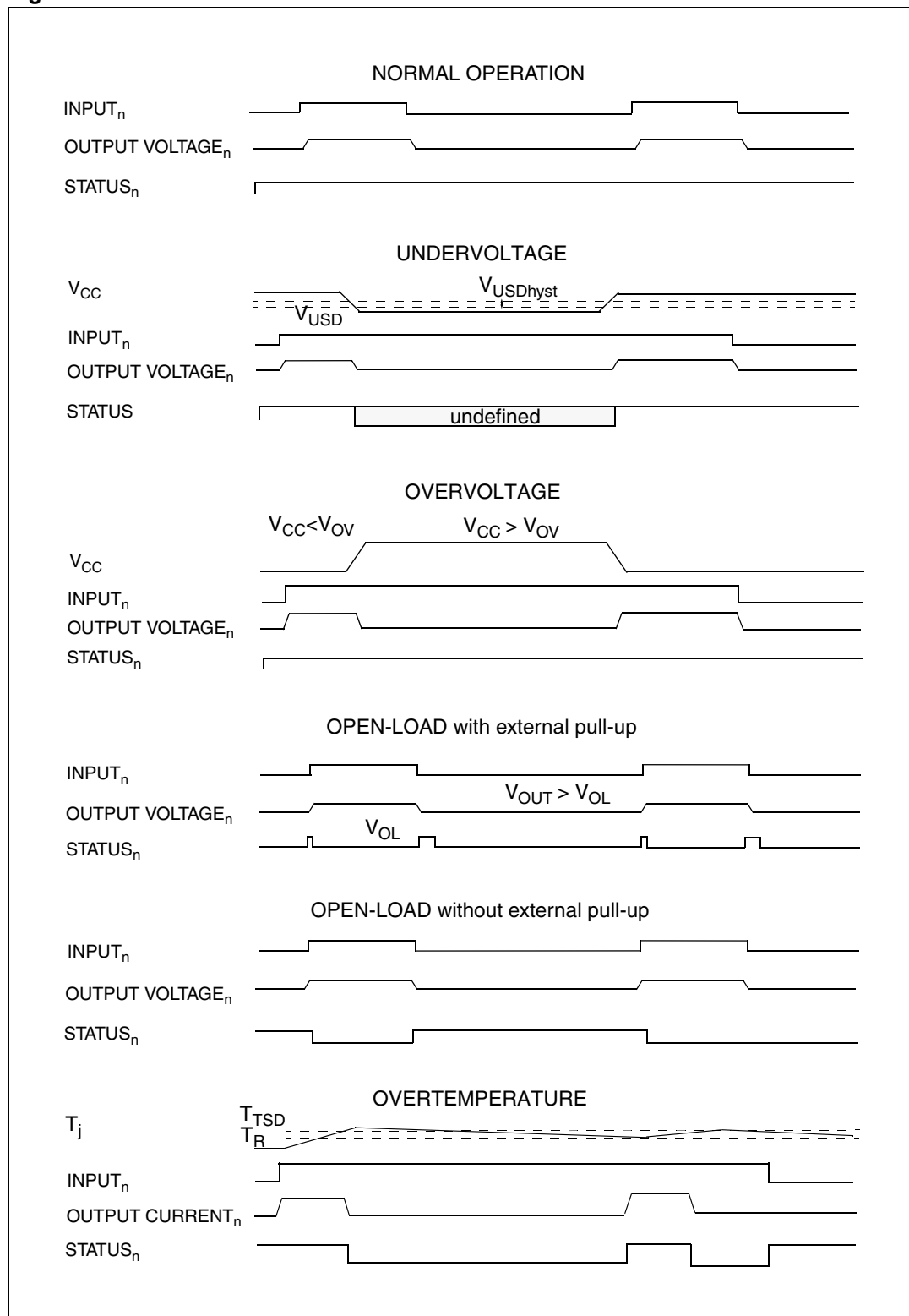
Figure 5. Waveforms
