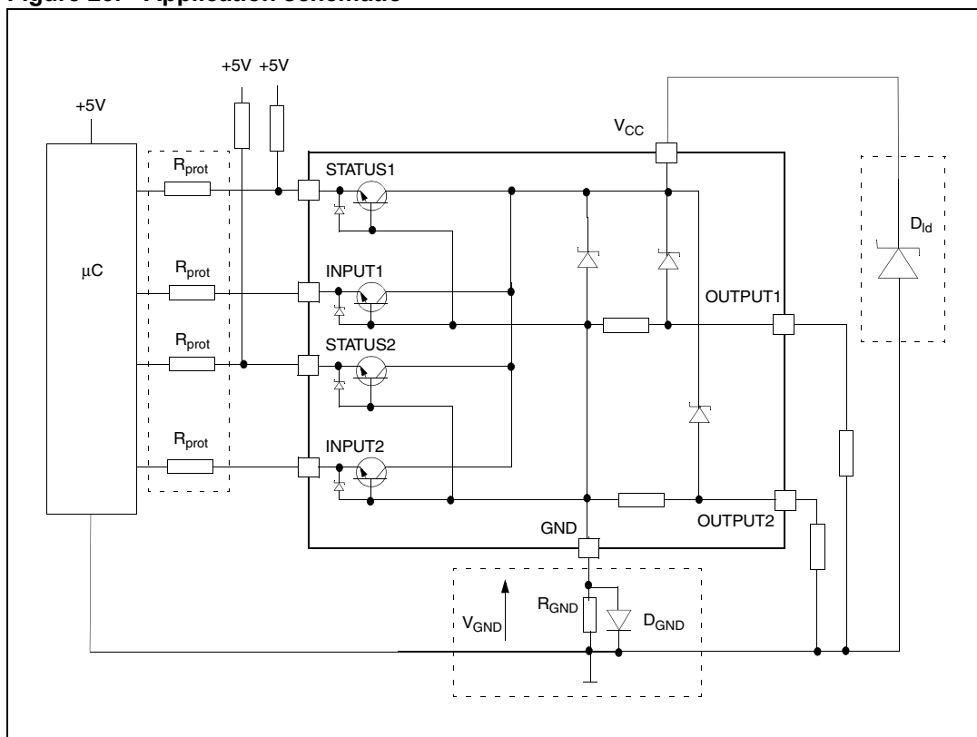
Figure 23. Application schematic
