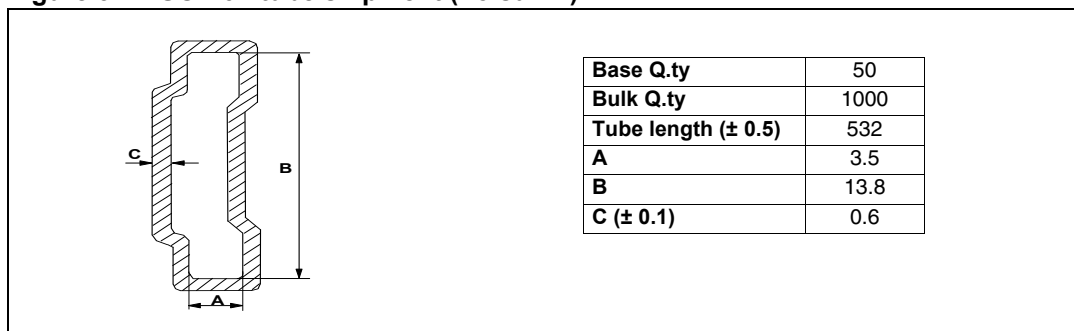
Figure 31. SO-16L tube shipment (no suffix)
