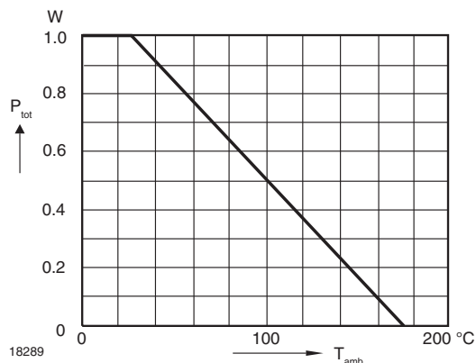
Fig. 1 - Admissible Power Dissipation vs. Ambient Temperature
