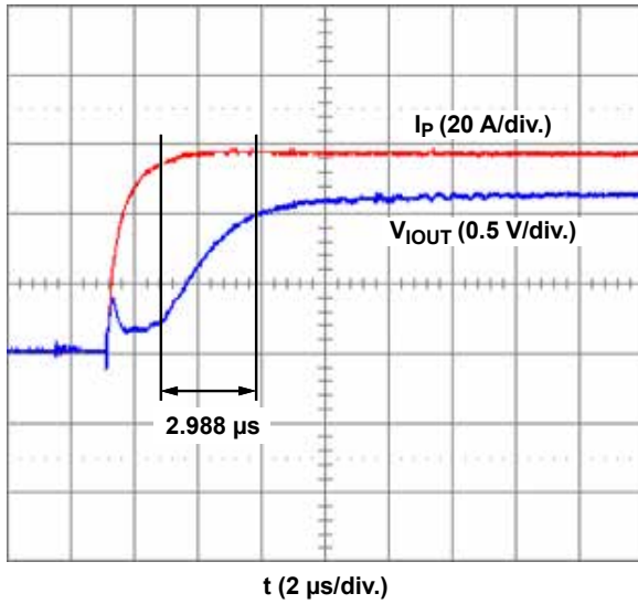
Rise Time
