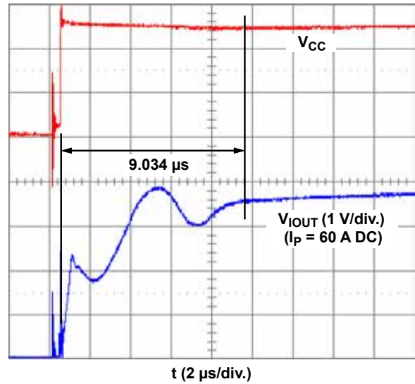
Power-on Delay
