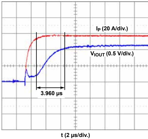
Response Time
