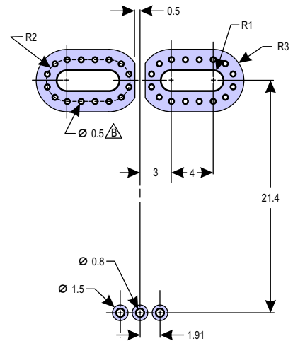
PCB Layout Reference View
