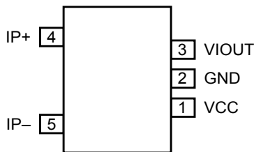
Pin-out Diagram
