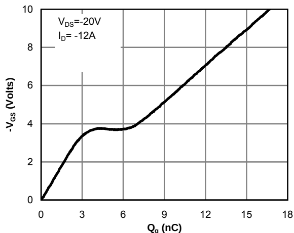
Figure 18: Gate-Charge Characteristics
