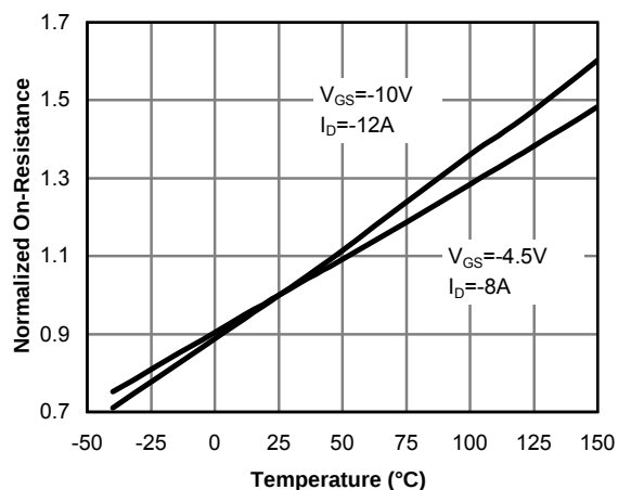
Figure 15: On-Resistance vs. Junction Temperature
