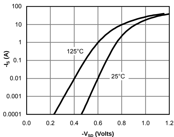
Figure 17: Body-Diode Characteristics
