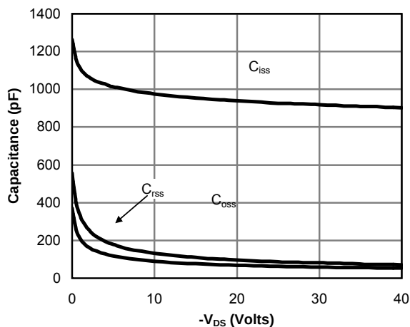
Figure 19: Capacitance Characteristics
