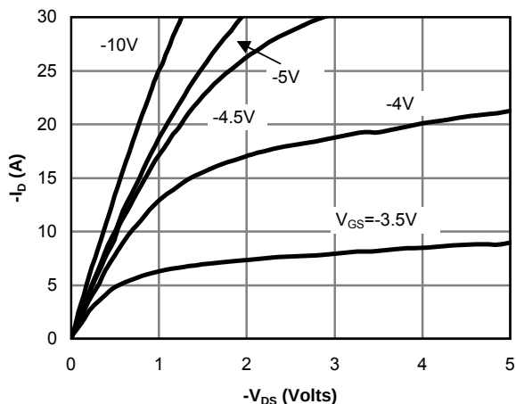
Figure 12: On-Region Characteristics
