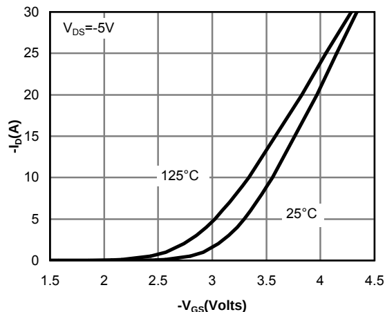
Figure 13: Transfer Characteristics
