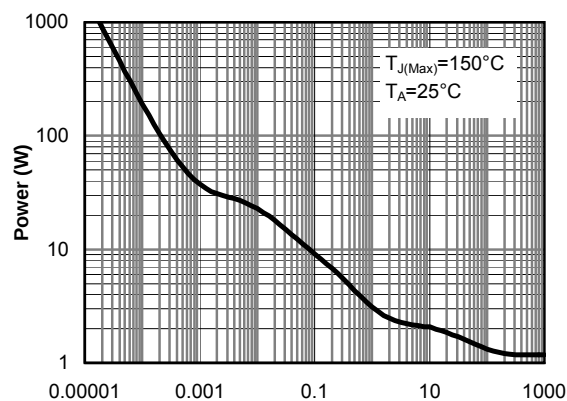
Figure 21: Single Pulse Power Rating Junction-to-Ambient (Note E)
