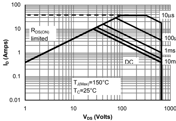
Figure 9: Maximum Forward Biased Safe Operating Area for AOT10N65 (Note F)
