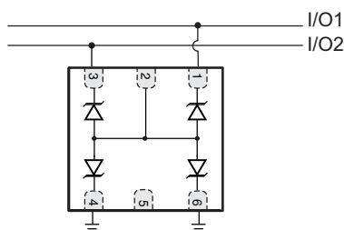
Bidirection Protection of Two Lines
