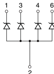
Circuit Diagram
