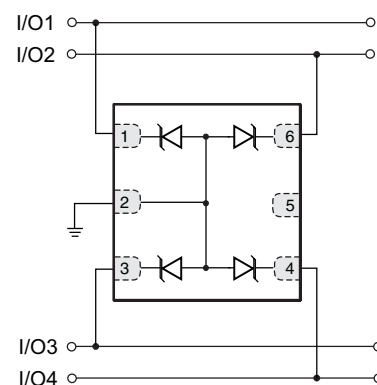
Protection of Four Unidirectional Lines
