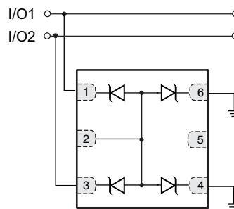
Protection of Two Bidirectional Lines
