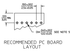
KINKED PIN OPTION SEE NOTE 5
