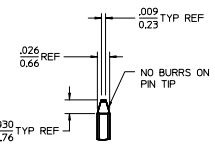
DETAIL X SCALE 5:1 SEE NOTE 10
