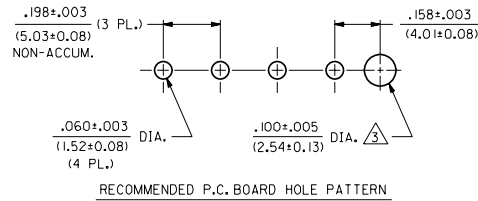
RECOMMENDED P.C. BOARD HOLE PATTERN
