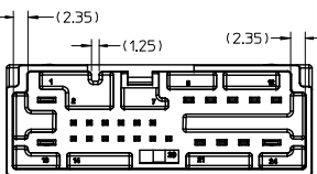
30700-4242 POLARIZATION 'C'
