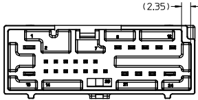
30700-4240 POLARIZATION 'A'
