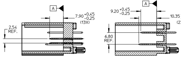
SECTION Y-Y
