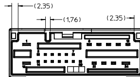
30700-4247 POLARIZATION 'C'
