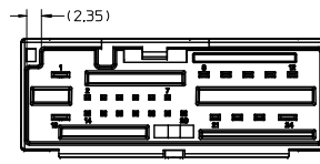
30700-4249 POLARIZATION 'B'
