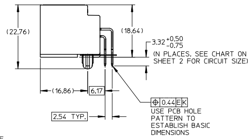
SECTION Z-Z
