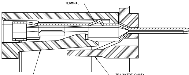
BLADE TERMINAL HOUSING CAVITY SECTION F-F TPA/INSERT CAVITY
