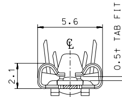
VIEW "A"
