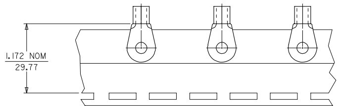
PARTS ON TAPE DOUBLE SPACED AS SHOWN
