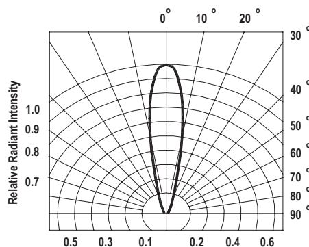
Figure 6. Radiation Diagram
