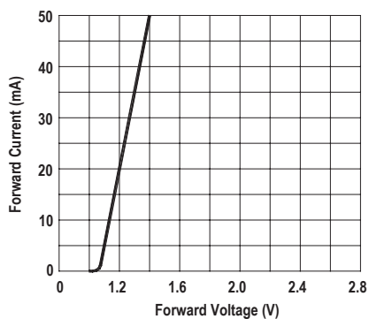
Figure 3. Forward Current Vs. Forward Voltage
