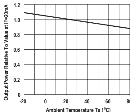
Figure 4. Relative Radiant Intensity Vs. Ambient Temperature
