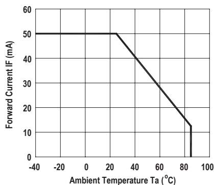
Figure 2. Forward Current Vs. Ambient Temperature
