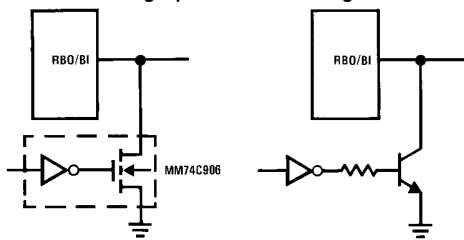
Blanking Input Connection Diagram
