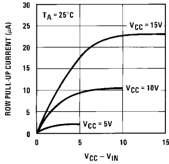
Typical I_{p} vs V_{IN} at Any Y Input
