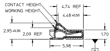
SECTION Z-Z
