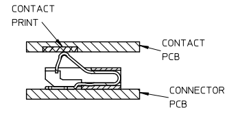
SECTION W-W
