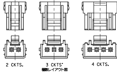
LAYOUT OF EACH CKTS.
