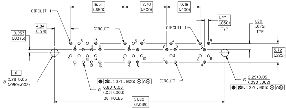
RECOMMENDED PC BOARD LAYOUT \triangle COMPONENT SIDE
