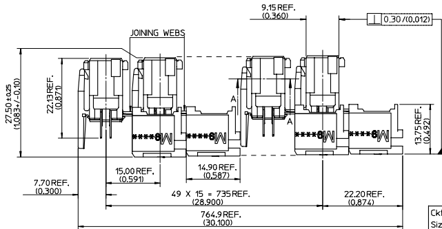
PARTIAL 1 Scale 2:1
