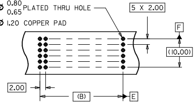
BACKPLANE HOLE PATTERN
