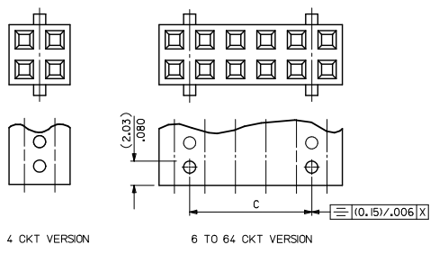
POLARISING BUTTON VERSION (90143-11** VERSION)
