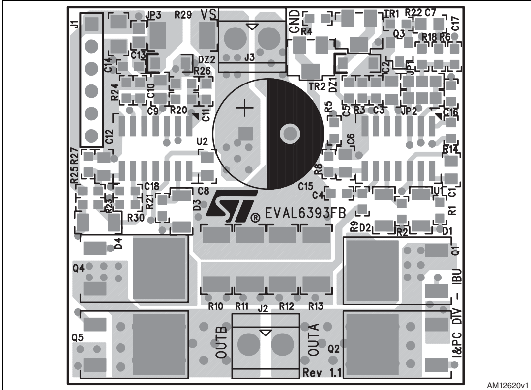
Figure 3. EVAL6393FB – layout (top layer)
