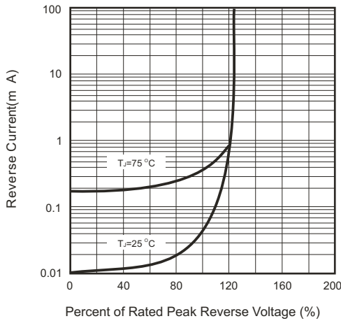
Fig.1 Reverse Characteristics
