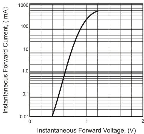
Fig.5 - Forward Characteristics
