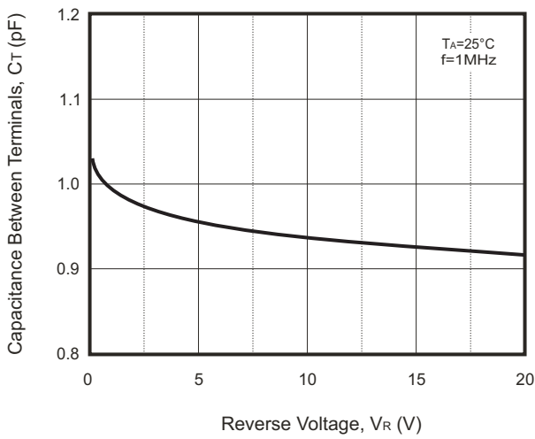
Fig.3 - Capacitance Characteristics
