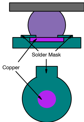
FIGURE 3. SMD
