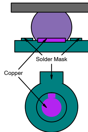
FIGURE 4. NSMD
